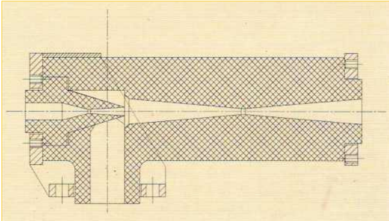
Ejector Assembly - Nozzle with Diffuser
