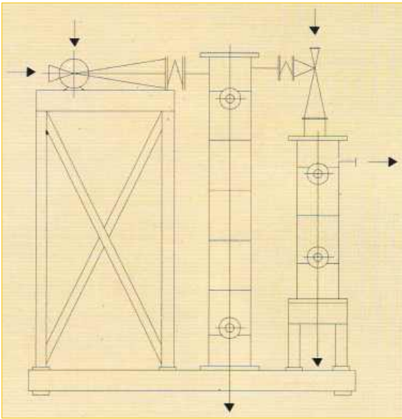
Ejector System with Intermidate Condenser
